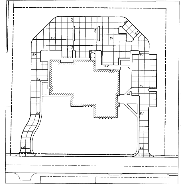
SUGGESTED JOINTING PLAN SCALE 1" = 50'
